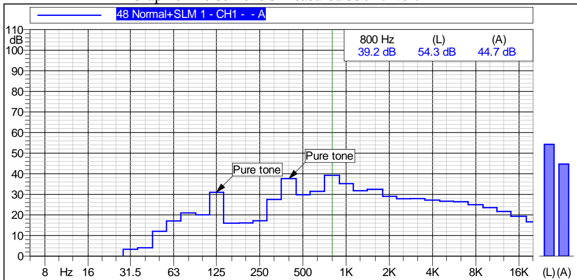
Figure A-2 Graph of Noise Levels Measured 330-ft North
