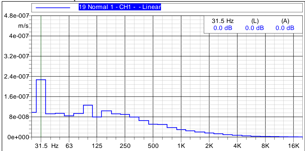
Figure C-6 Graph of Vibration Velocities Measured 2640-ft North
