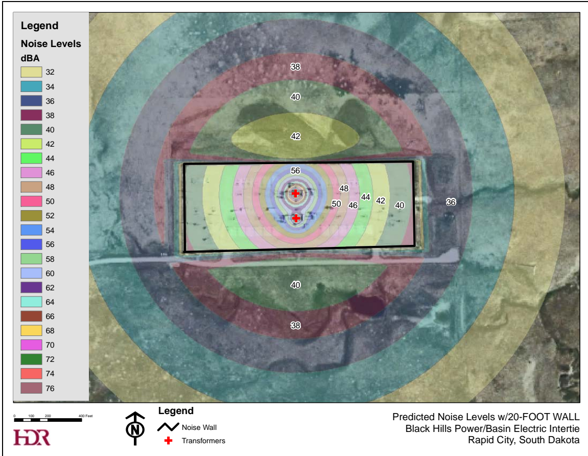
Figure 7-3 Predicted Noise Levels – 20-foot Wall
