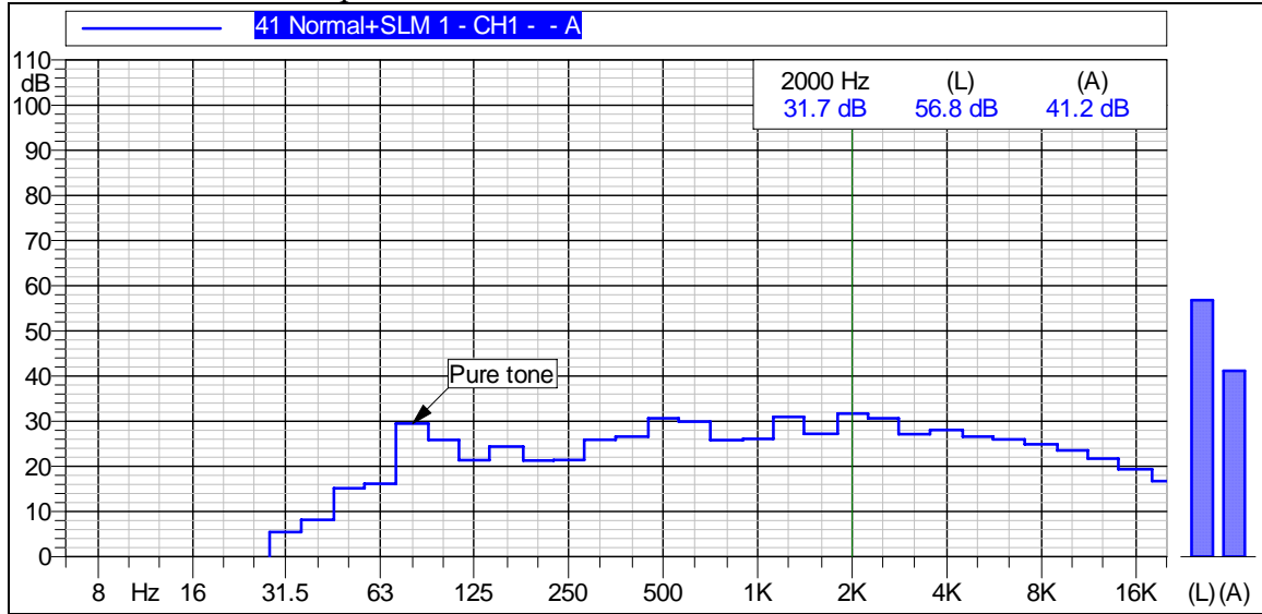
Figure A-16 Graph of Noise Levels Measured 1320-ft East
