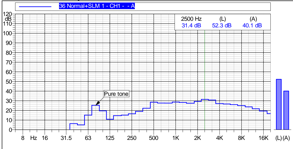
Figure A-23 Graph of Noise Levels Measured 1980-ft West
