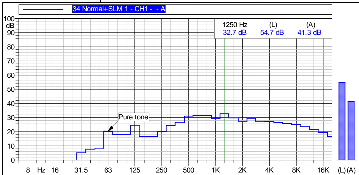
Figure A-21 Graph of Noise Levels Measured 660-ft East
