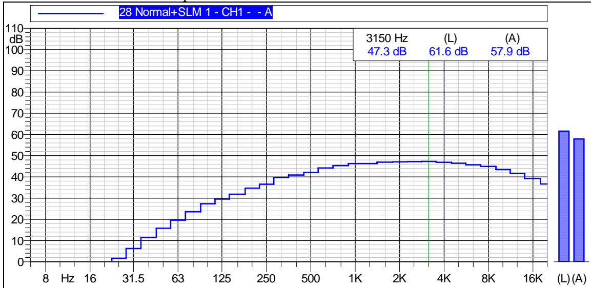
Figure A-9 Graph of Noise Levels Measured 660-ft South
