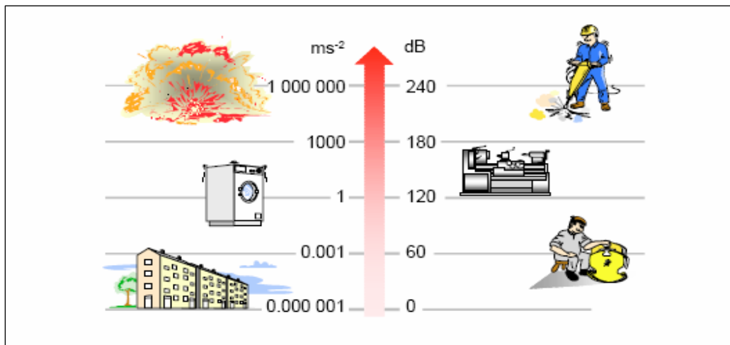
Figure 2-7 Range of Common Vibration Sources
