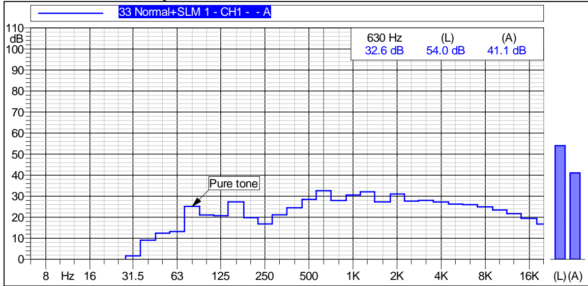
Figure A-20 Graph of Noise Levels Measured 330-ft East
