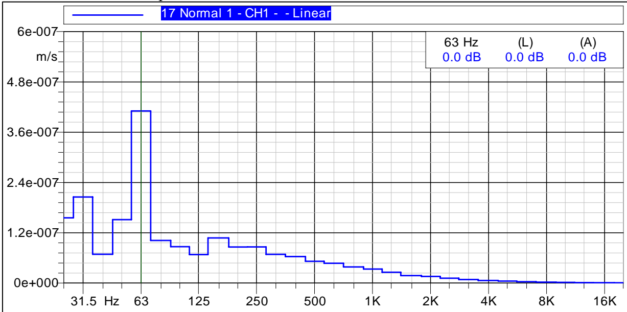
Figure C-16 Graph of Vibration Velocities Measured 1980-ft East
