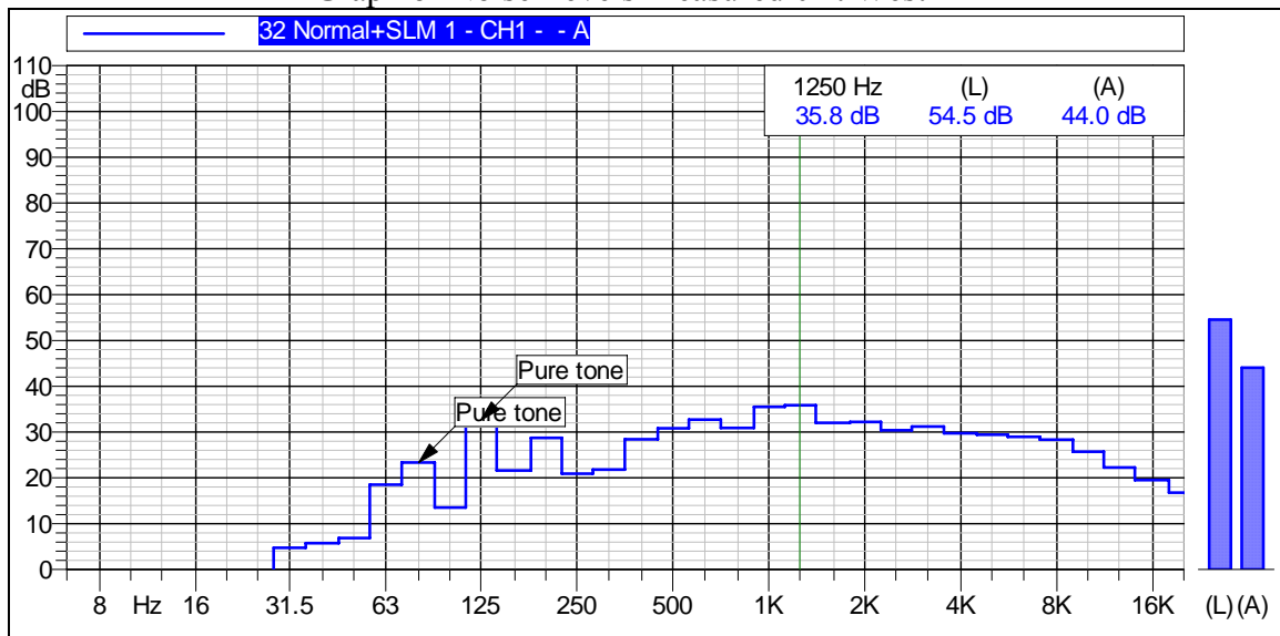
Figure A-19 Graph of Noise Levels Measured 0-ft West
