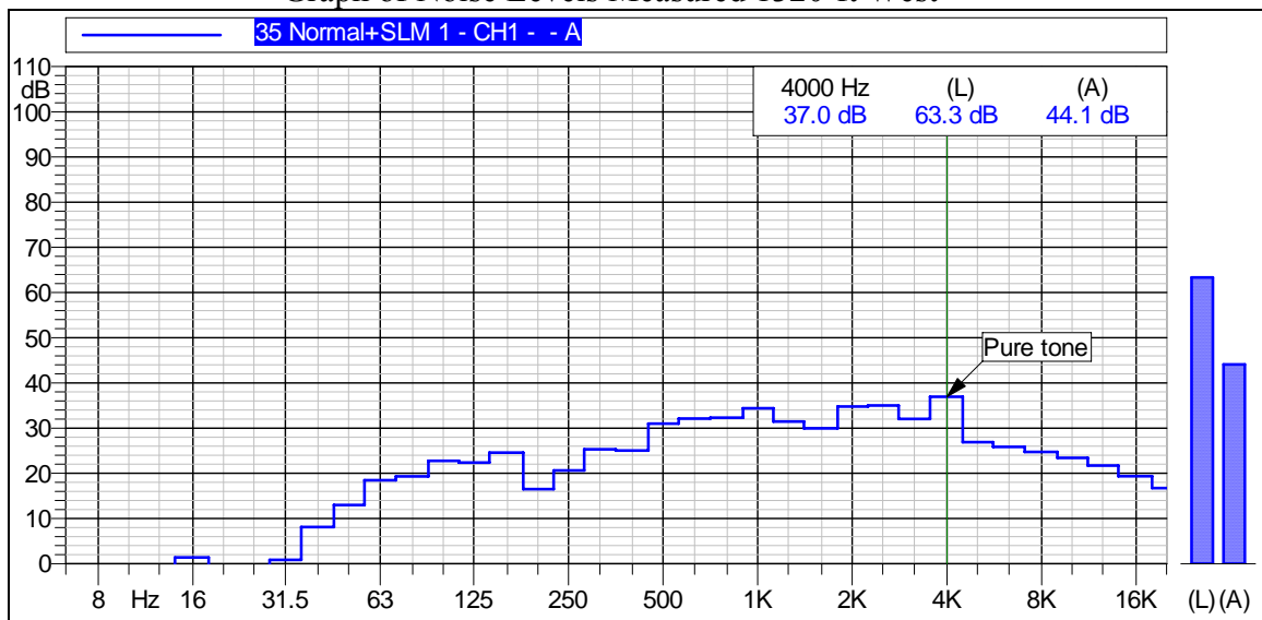
Figure A-22 Graph of Noise Levels Measured 1320-ft West
