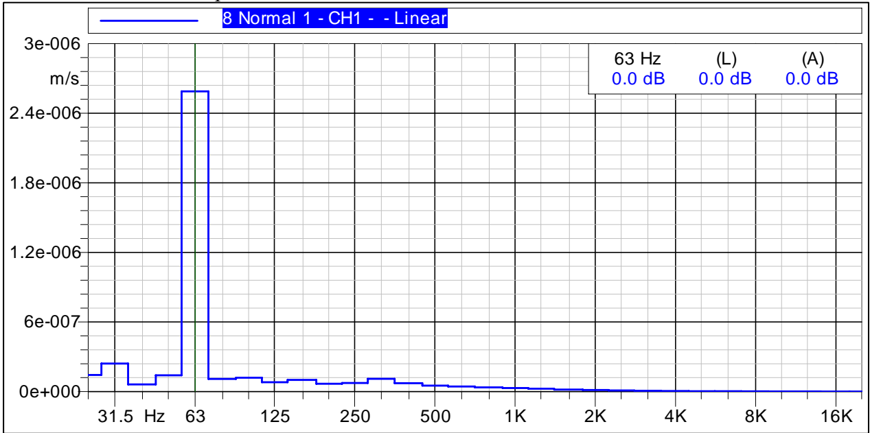
Figure C-19 Graph of Vibration Velocities Measured 330-ft West
