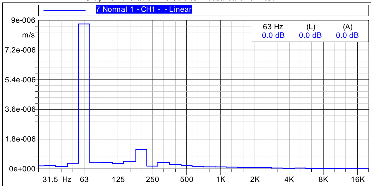
Figure C-18 Graph of Vibration Velocities Measured 0-ft West
