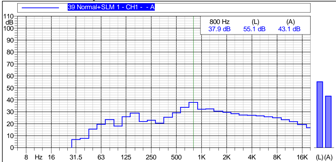
Figure A-14 Graph of Noise Levels Measured 330-ft East
