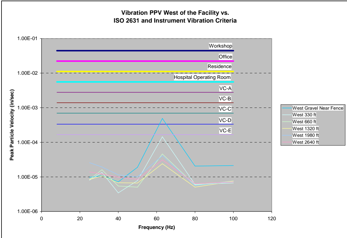
Figure 6-4 Vibration PPV West of the Facility
