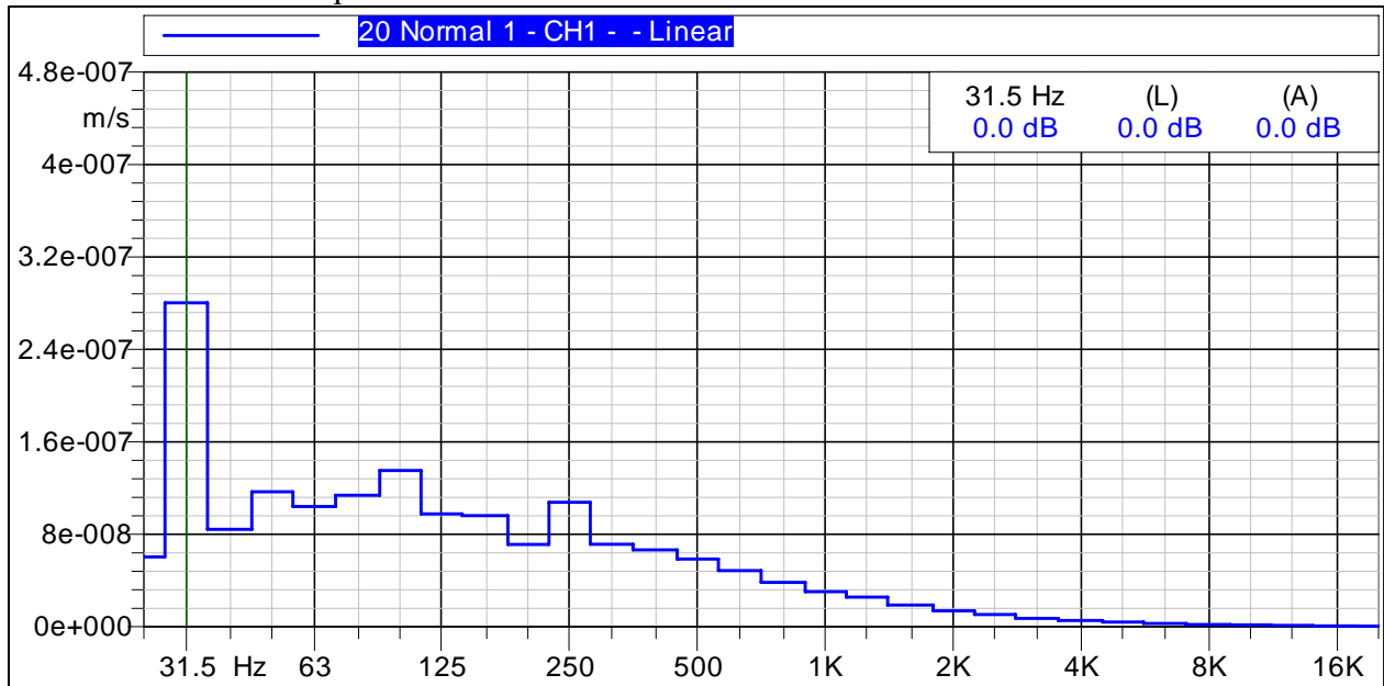
Figure C-5 Graph of Vibration Velocities Measured 1980-ft North
