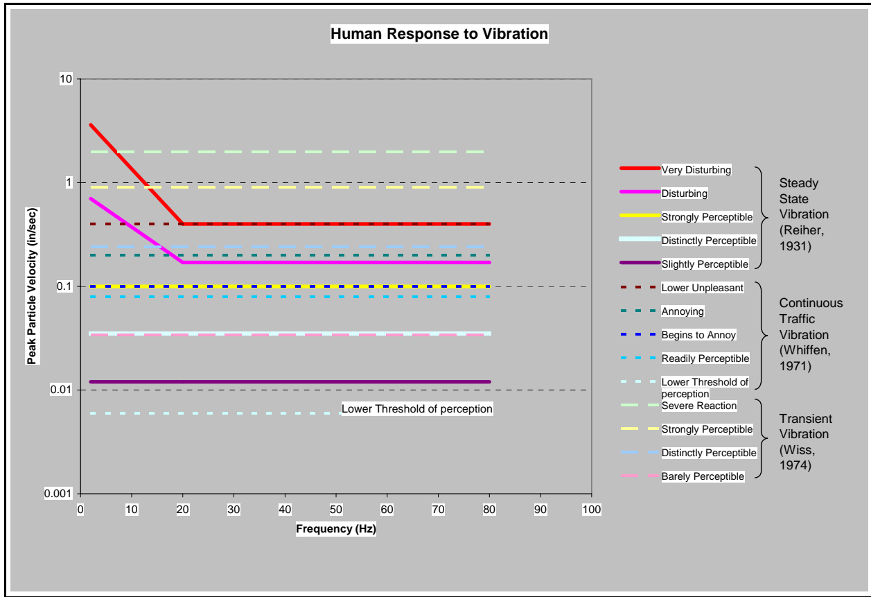
Figure 4-1 Human Response to Vibration Criteria
