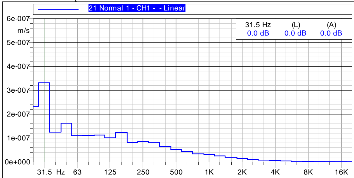
Figure C-4 Graph of Vibration Velocities Measured 1320-ft North
