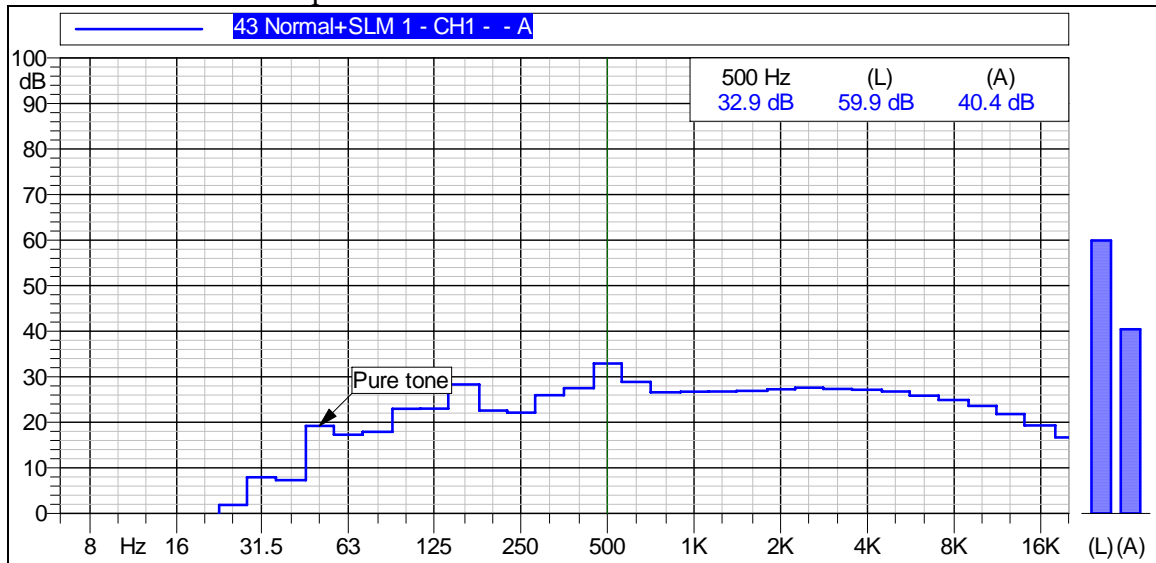
Figure A-18 Graph of Noise Levels Measured 2640-ft East
