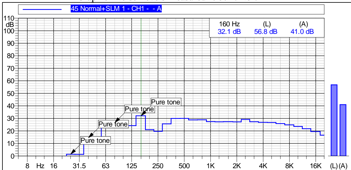
Figure A-5 Graph of Noise Levels Measured 1980-ft North
