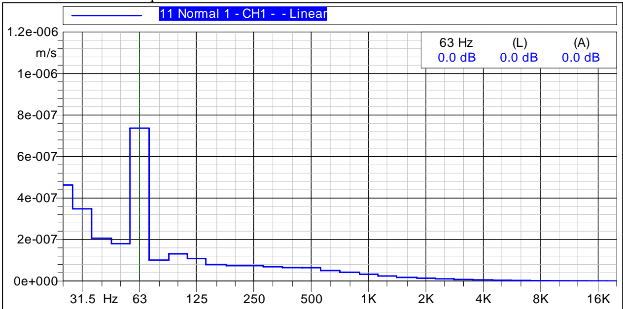
Figure C-22 Graph of Vibration Velocities Measured 1980-ft West
