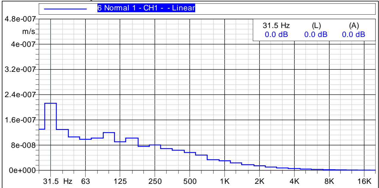
Figure C-12 Graph of Vibration Velocities Measured 1980-ft South
