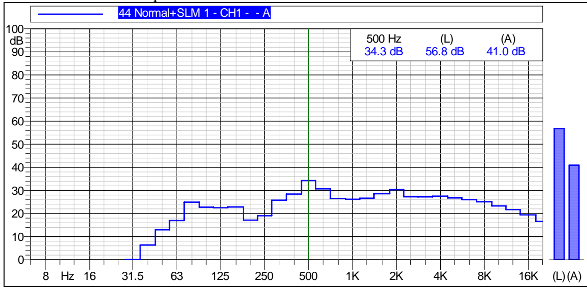
Figure A-6 Graph of Noise Levels Measured 2640-ft North
