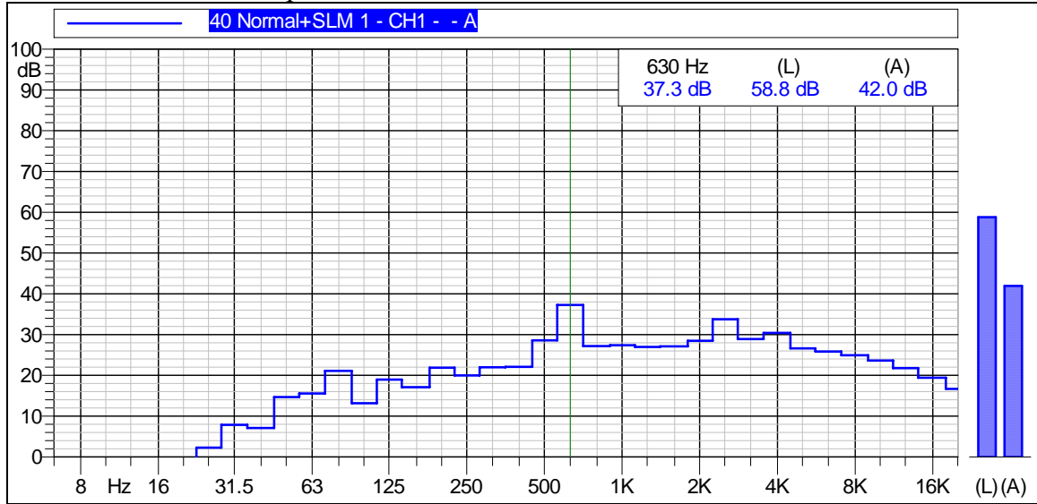
Figure A-15 Graph of Noise Levels Measured 660-ft East
