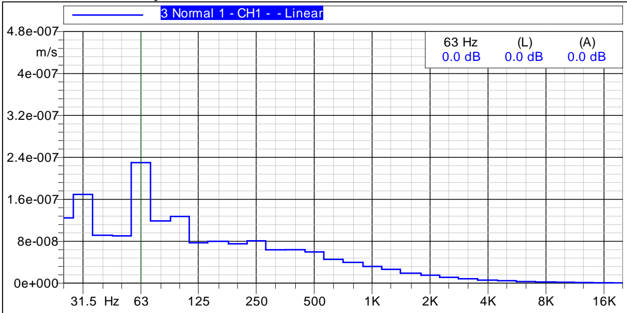
Figure C-9 Graph of Vibration Velocities Measured 660-ft South
