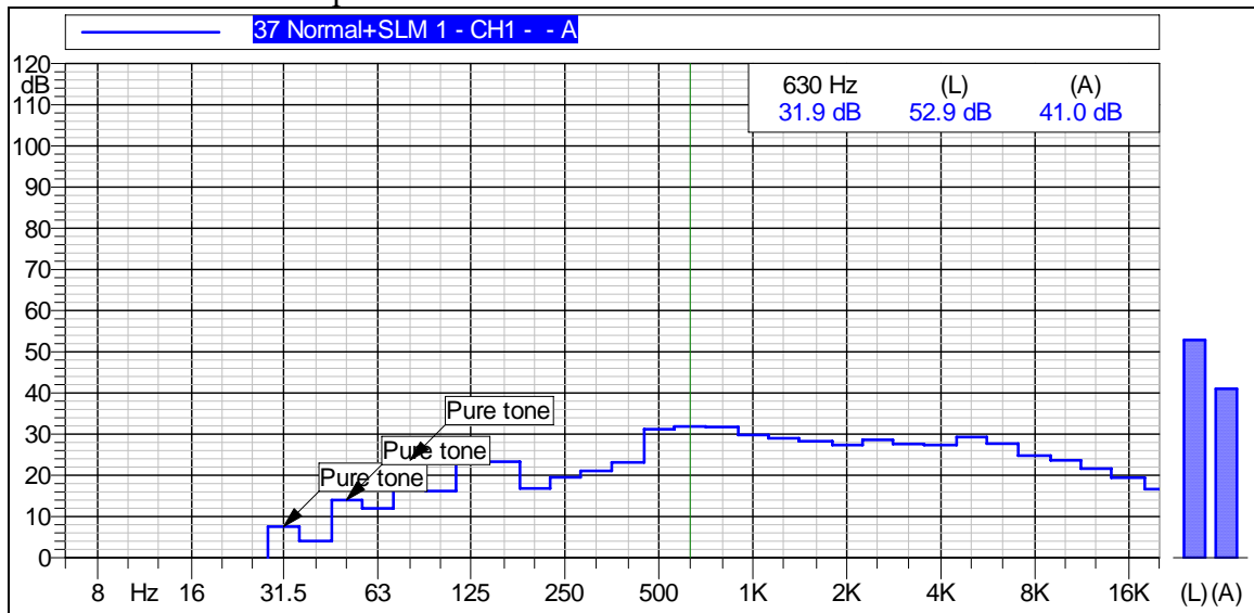
Figure A-24 Graph of Noise Levels Measured 2640-ft West
