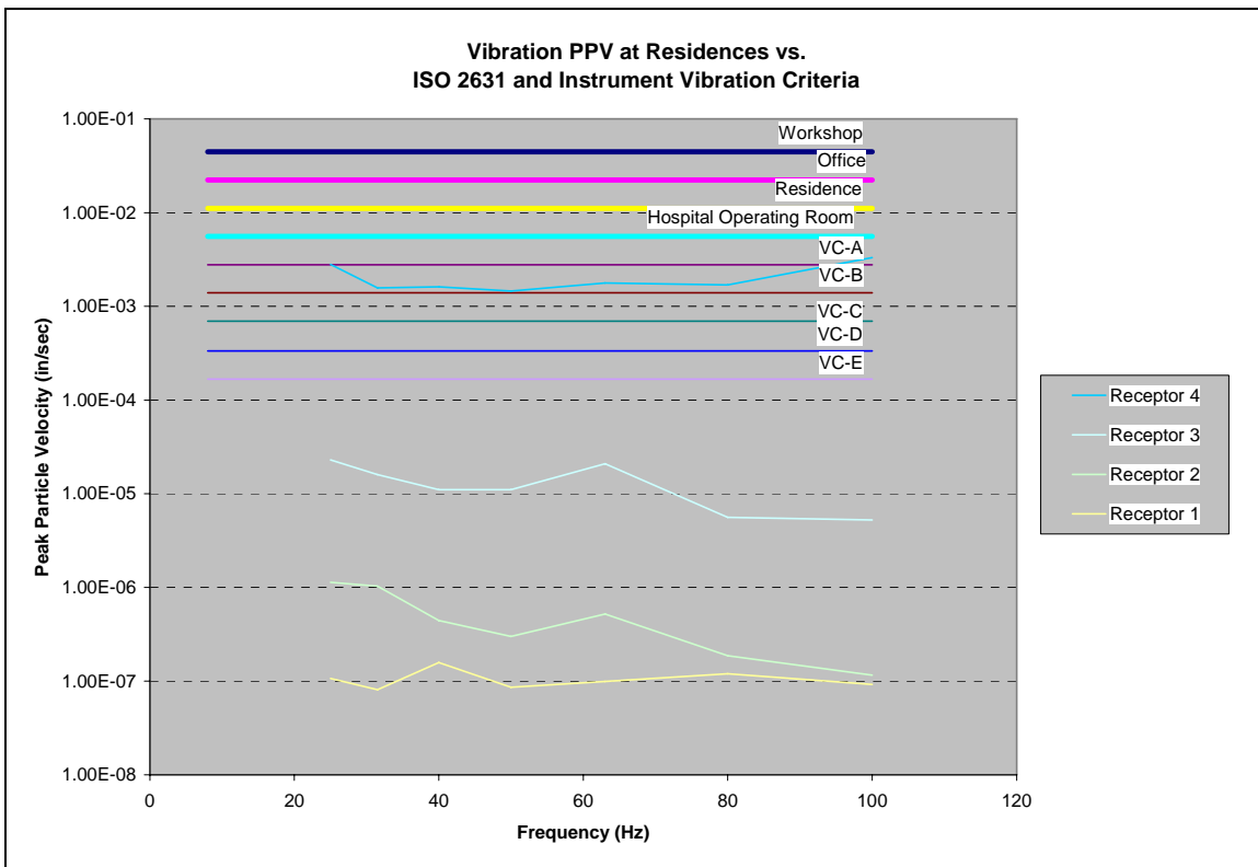
Figure 6-5 Vibration PPV at Residences
