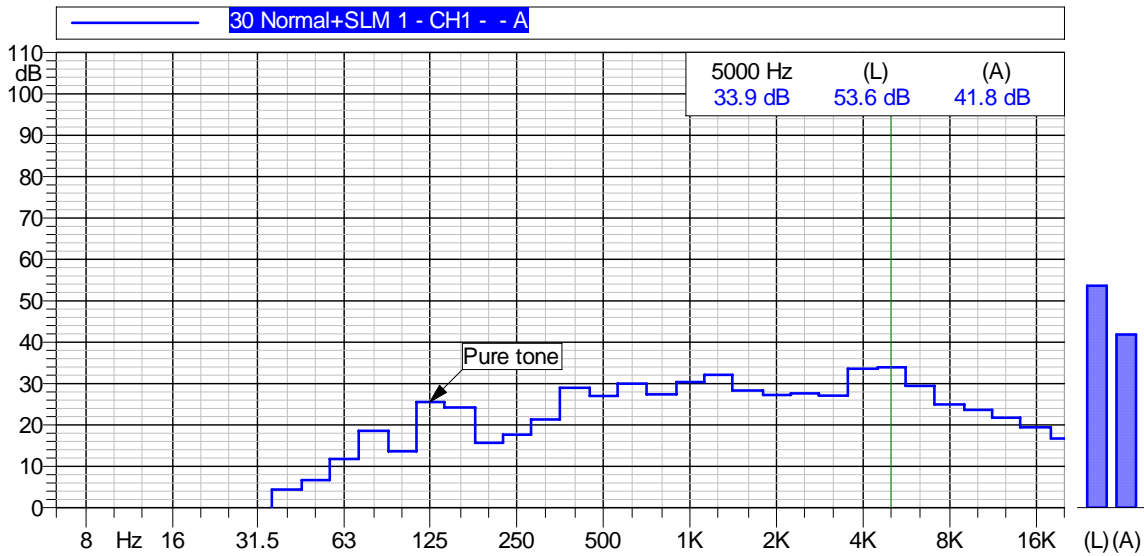
Figure A-11 Graph of Noise Levels Measured 1980-ft South
