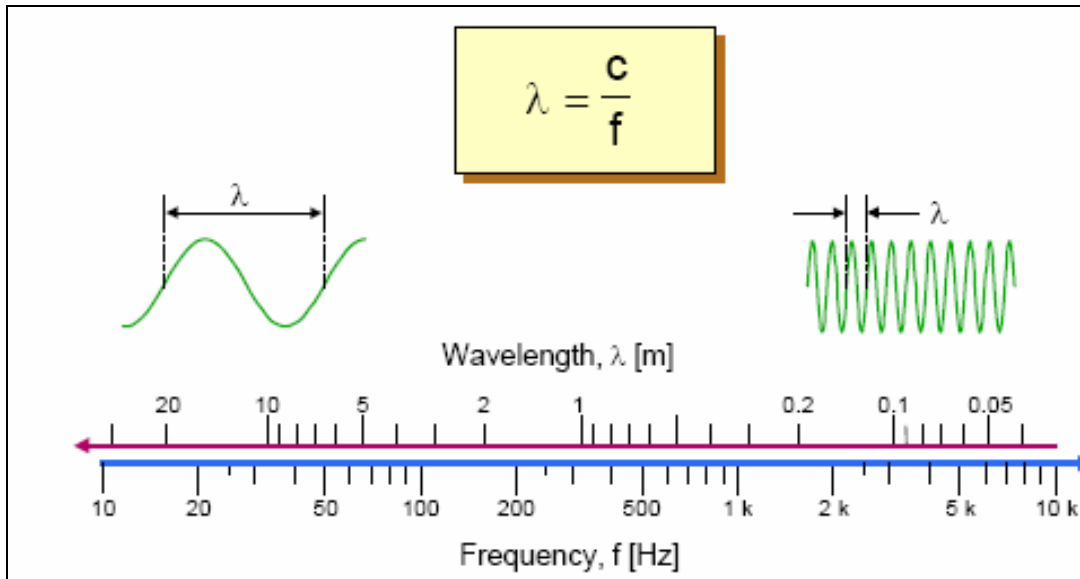
Figure 2-6 Relationship between Frequency and Wavelength
