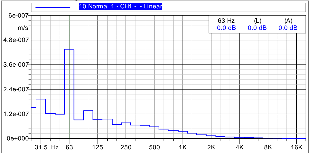
Figure C-21 Graph of Vibration Velocities Measured 1320-ft West
