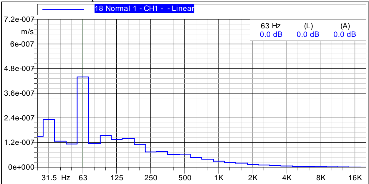
Figure C-17 Graph of Vibration Velocities Measured 2640-ft East
