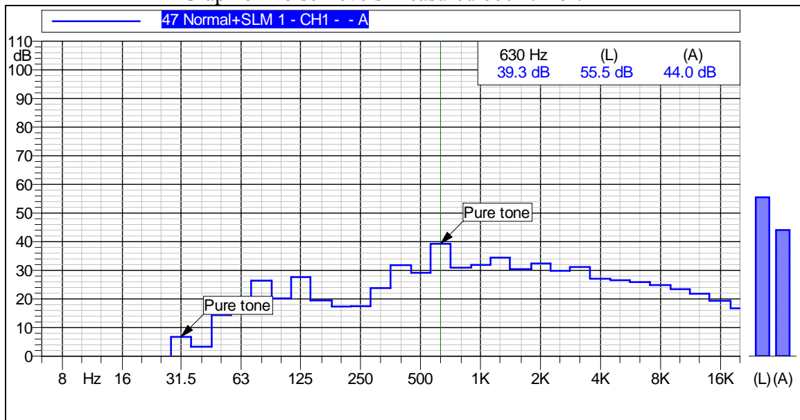
Figure A-3 Graph of Noise Levels Measured 660-ft North
