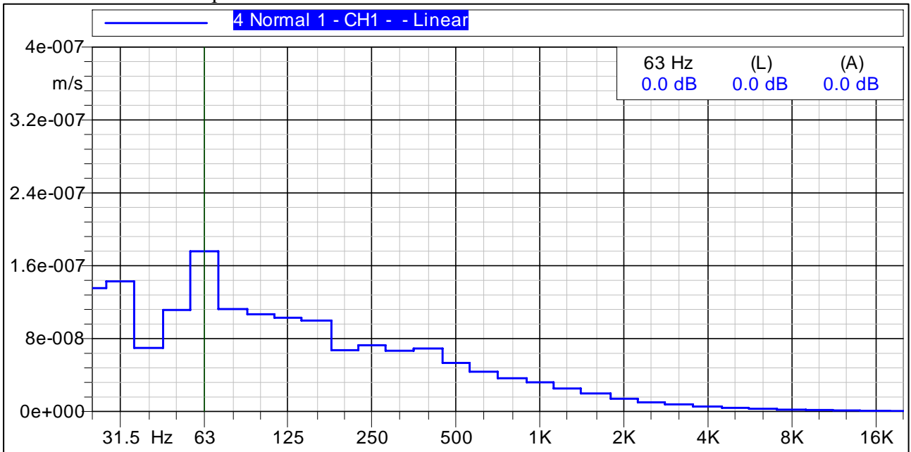
Figure C-10 Graph of Vibration Velocities Measured 1320-ft South
