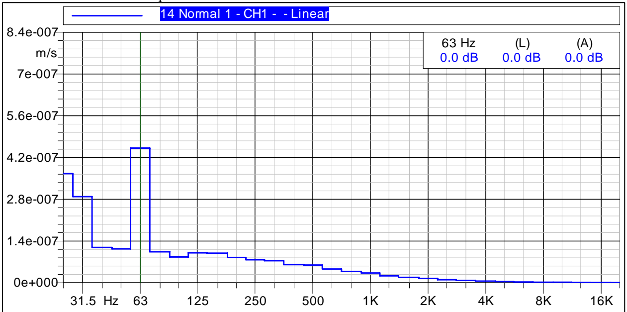
Figure C-14 Graph of Vibration Velocities Measured 330-ft East
