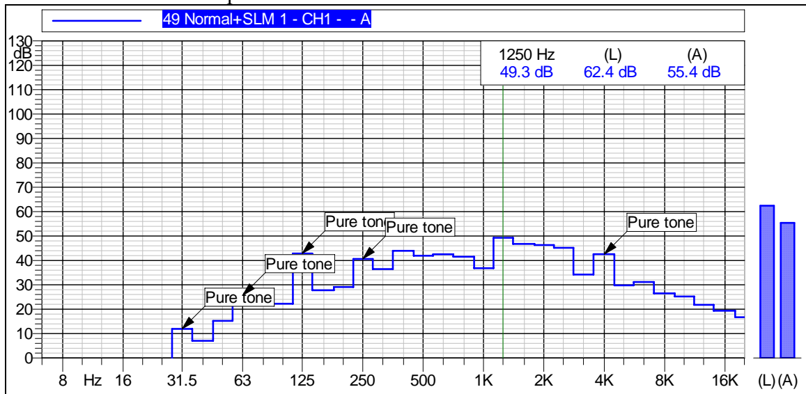
Figure A-1 Graph of Noise Levels Measured 0-ft North
