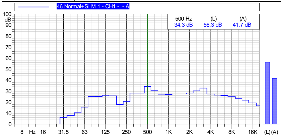
Figure A-4 Graph of Noise Levels Measured 1320-ft North
