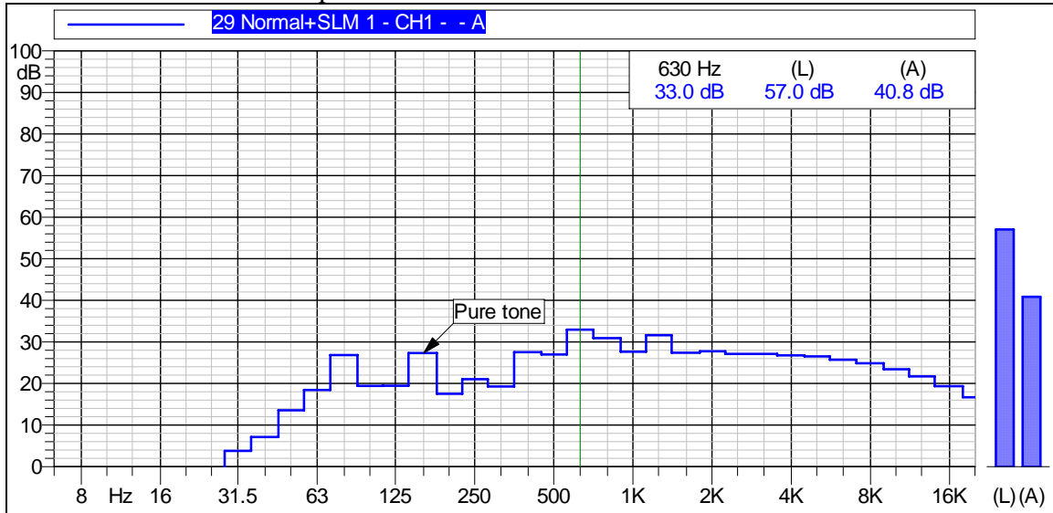
Figure A-10 Graph of Noise Levels Measured 1320-ft South
