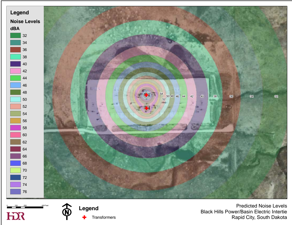
Figure 7-1 Predicted Noise Levels – Base Condition
