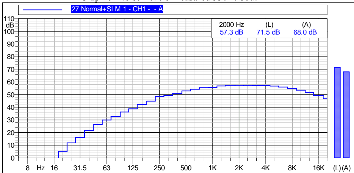
Figure A-8 Graph of Noise Levels Measured 330-ft South
