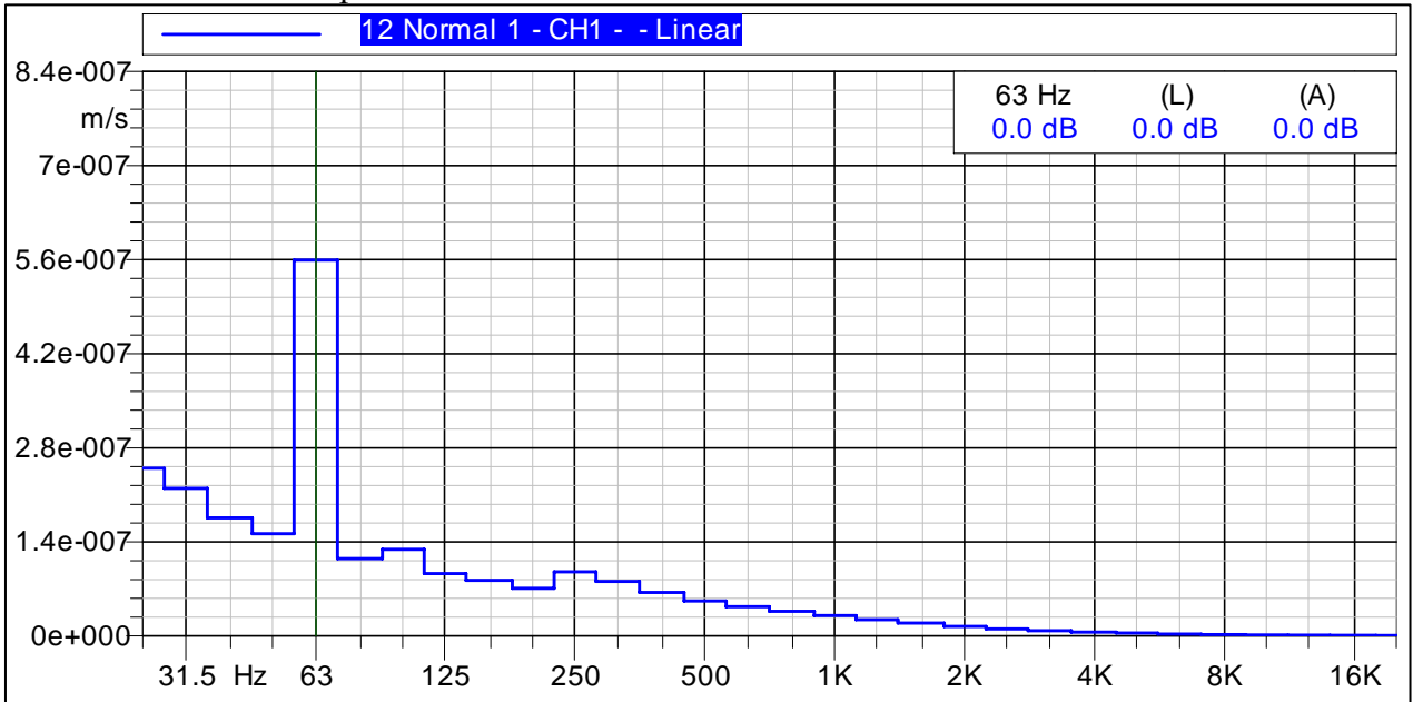
Figure C-23 Graph of Vibration Velocities Measured 2640-ft West
