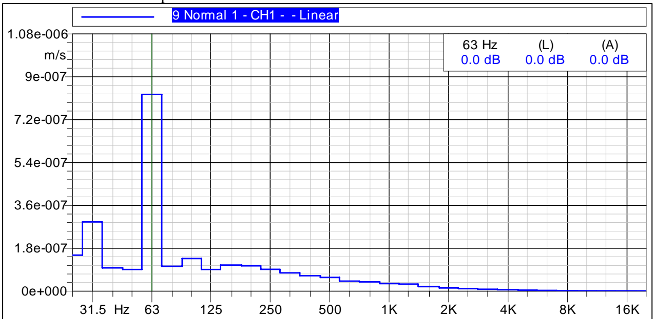
Figure C-20 Graph of Vibration Velocities Measured 660-ft West
