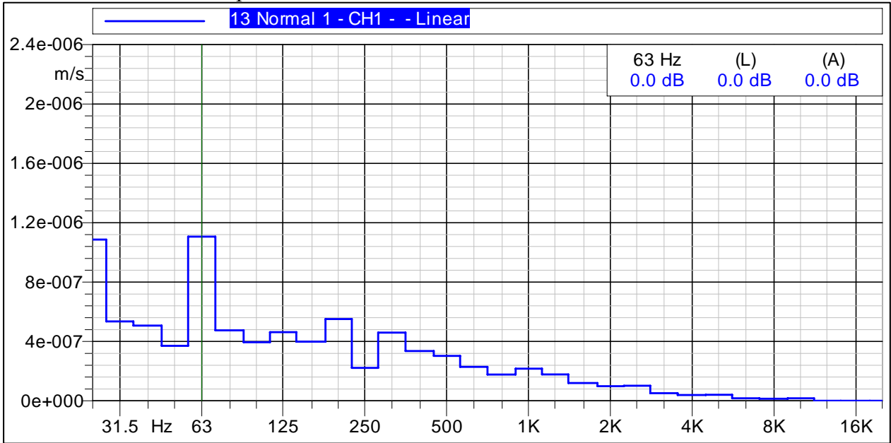
Figure C-13 Graph of Vibration Velocities Measured 0-ft East
