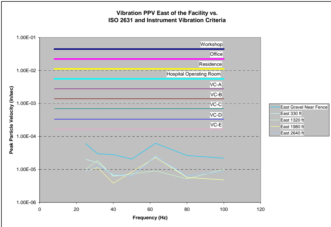
Figure 6-3 Vibration PPV East of the Facility
