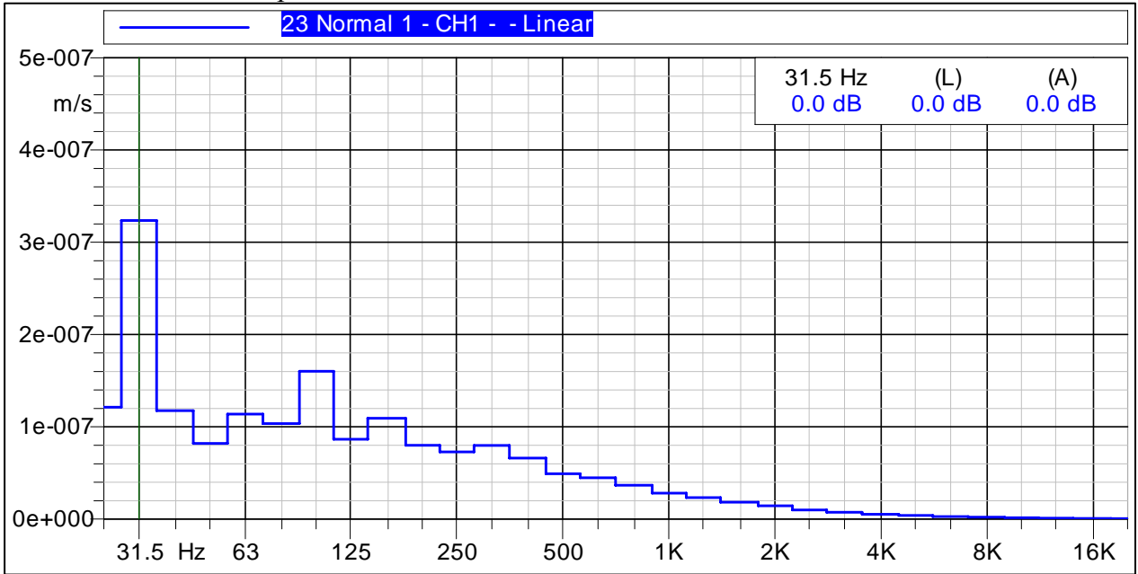
Figure C-2 Graph of Vibration Velocities Measured 330-ft North
