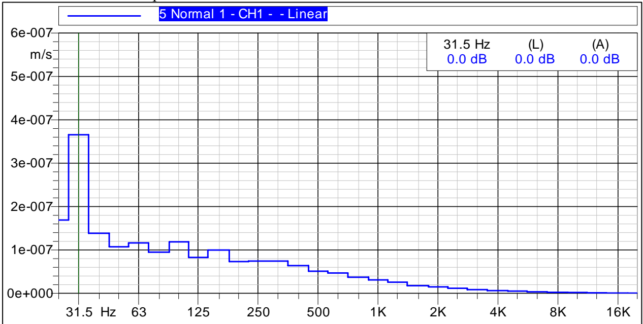
Figure C-11 Graph of Vibration Velocities Measured 1980-ft South
