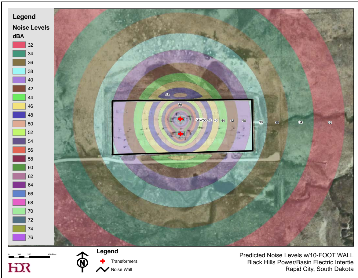
Figure 7-2 Predicted Noise Levels – 10-foot Wall
