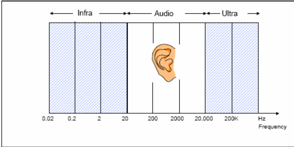
Figure 2-3 Sound Frequencies
