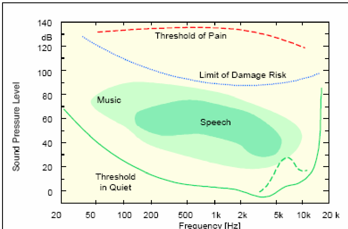
Figure 2-5 Auditory Field
