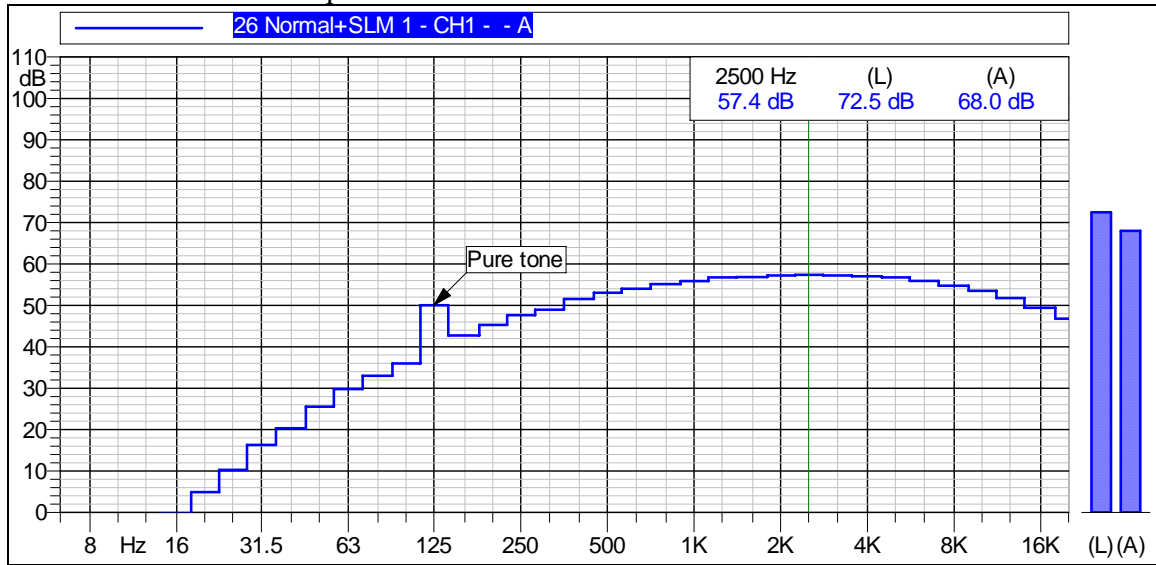
Figure A-7 Graph of Noise Levels Measured 0-ft South
