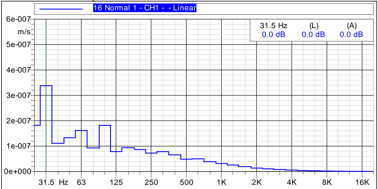
Figure C-15 Graph of Vibration Velocities Measured 1320-ft East
