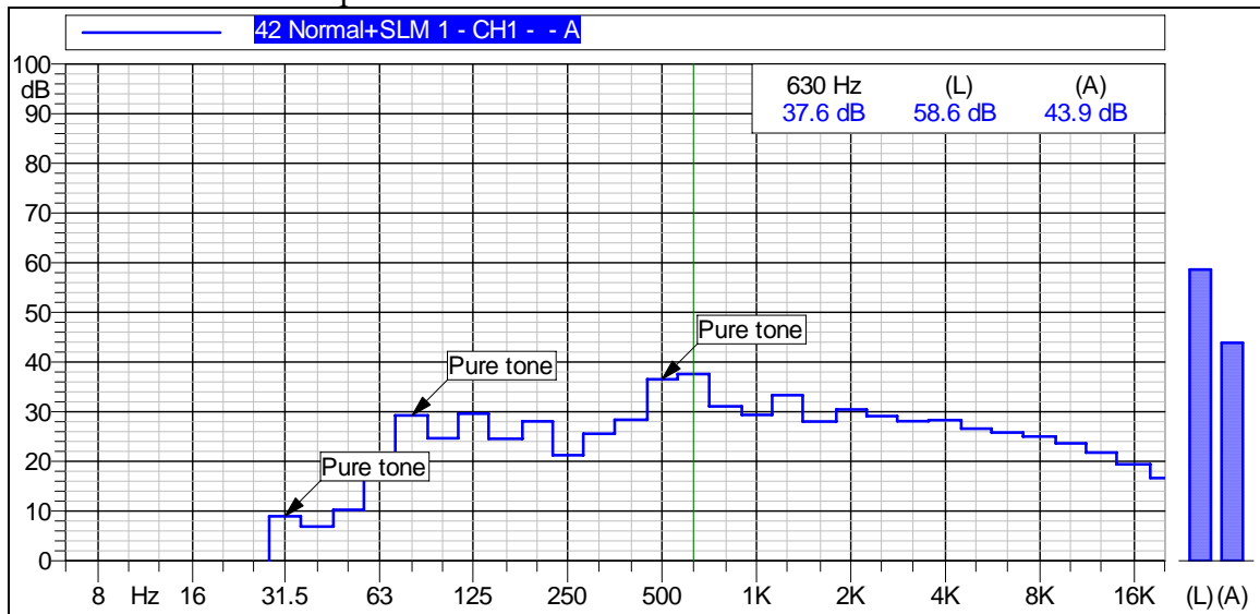
Figure A-17 Graph of Noise Levels Measured 1980-ft East
