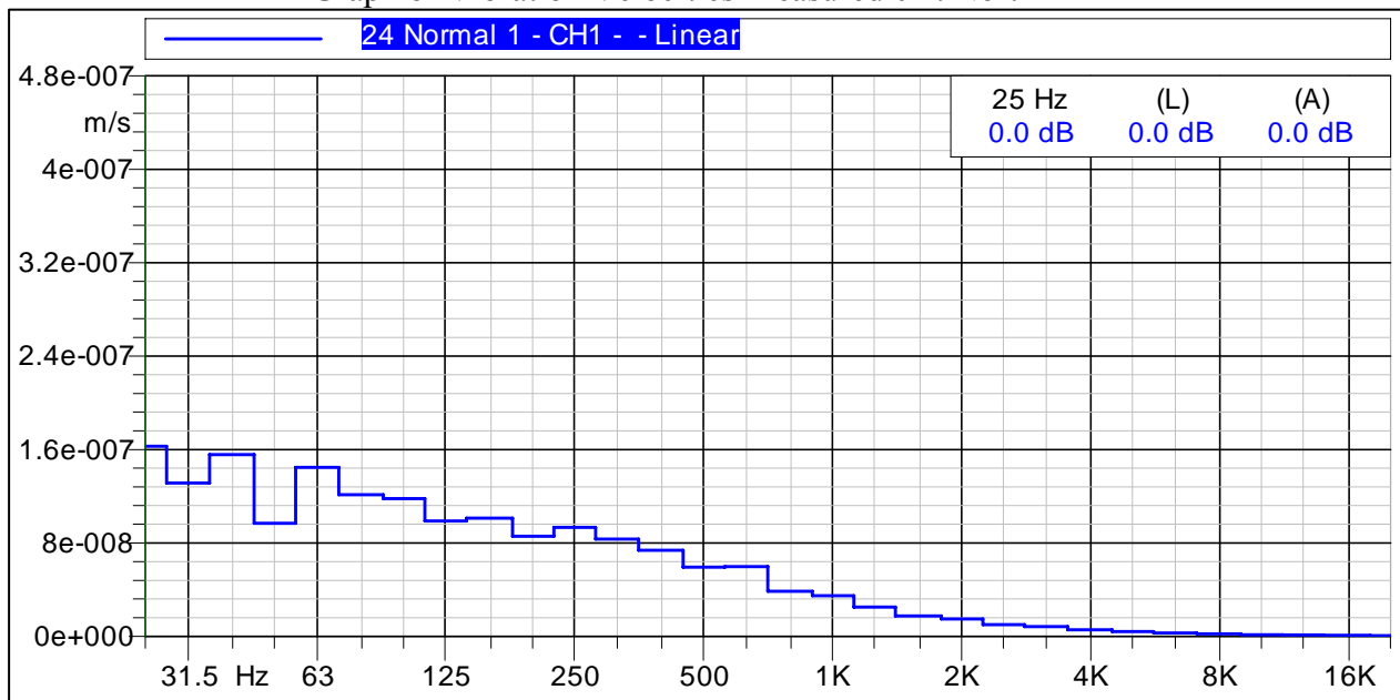
Figure C-1 Graph of Vibration Velocities Measured 0-ft North
