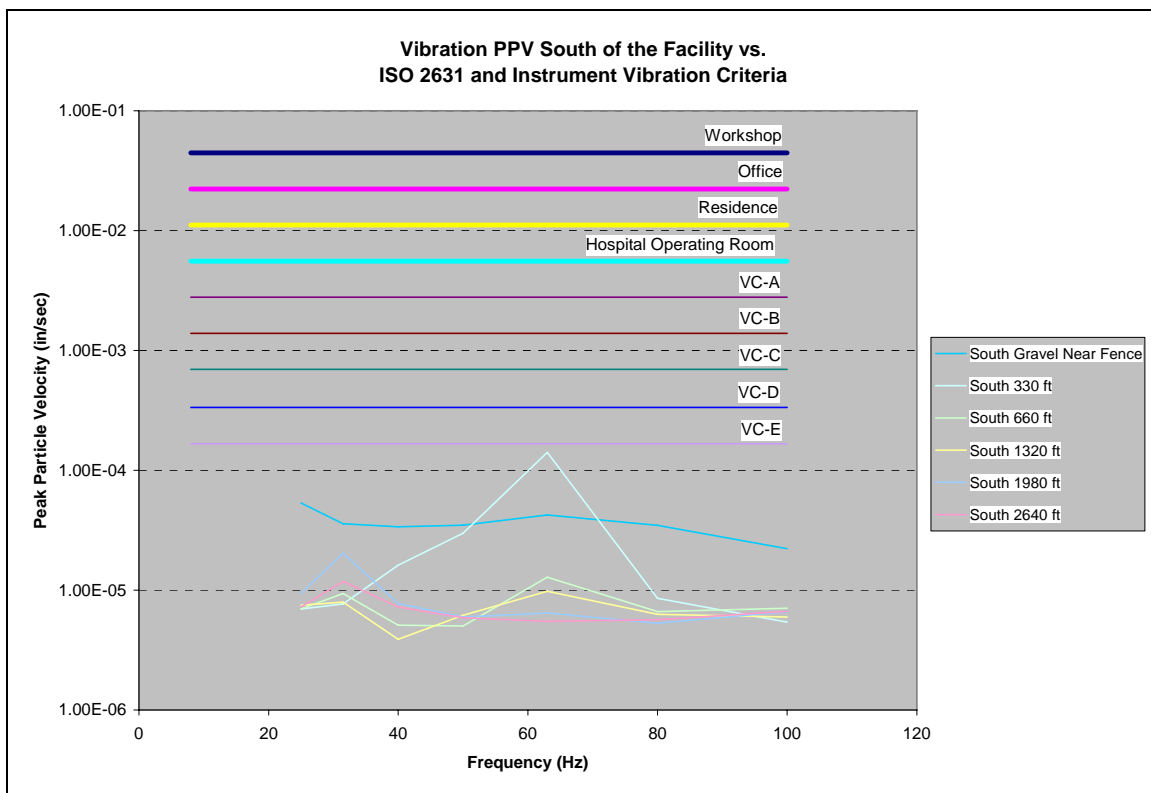
Figure 6-2 Vibration PPV South of the Facility
