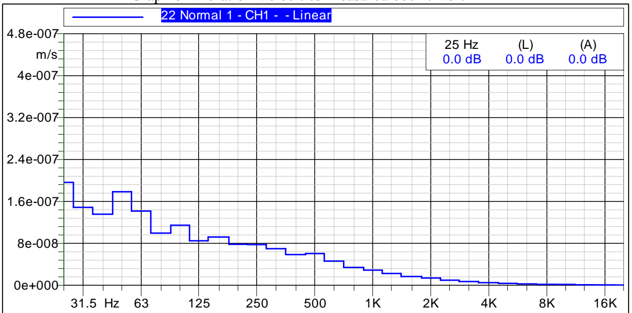
Figure C-3 Graph of Vibration Velocities Measured 660-ft North
