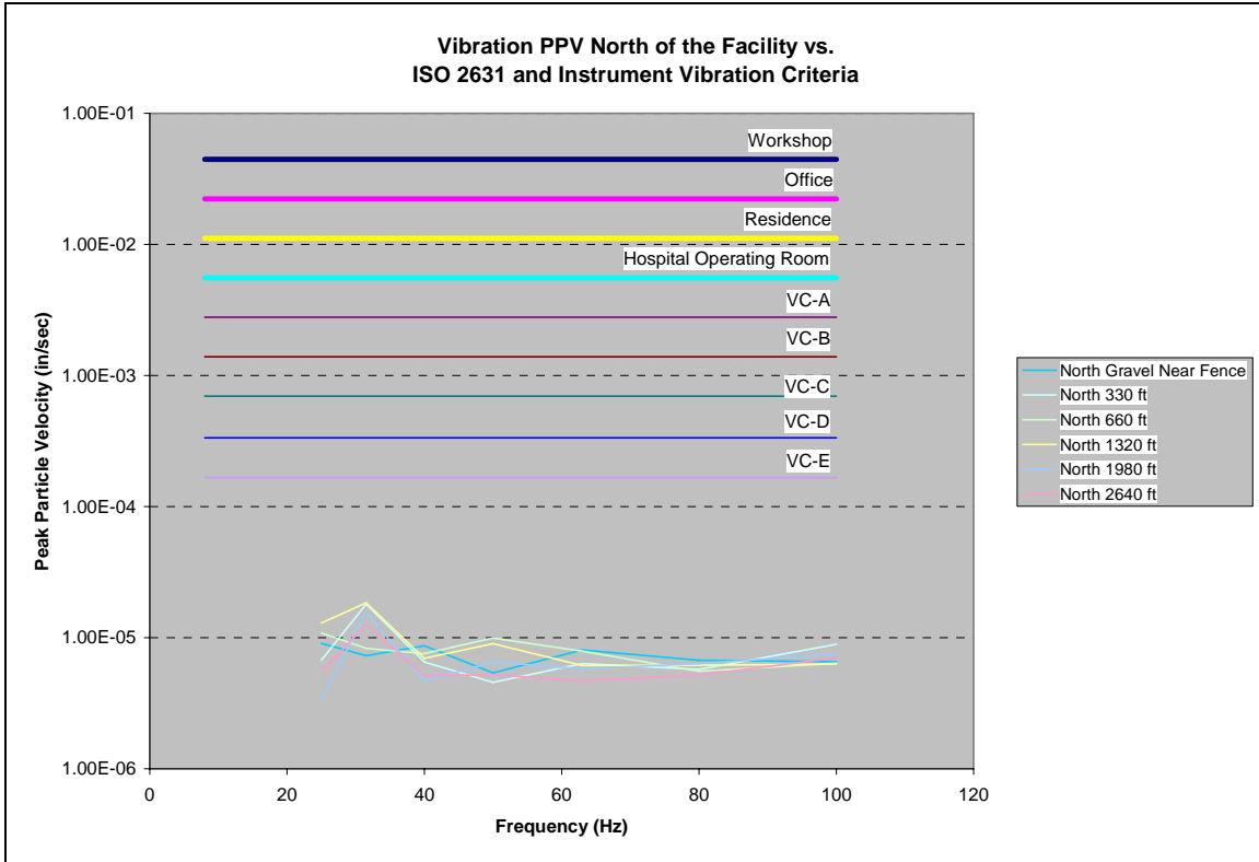
Figure 6-1 Vibration PPV North of the Facility
